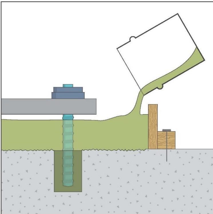
Figure 8 - Grouting under the plate with multiple buckets
