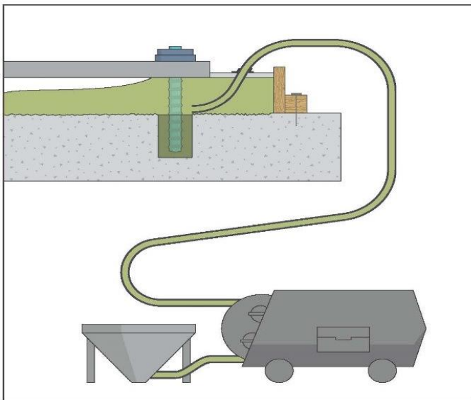
Figure 6 - Grouting under the plate with a pump
