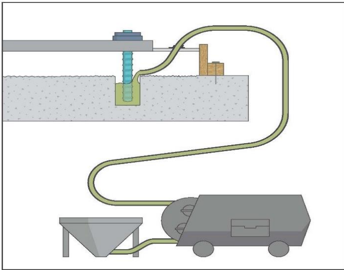
Figure 5 - Filling bolt pockets with a pump
