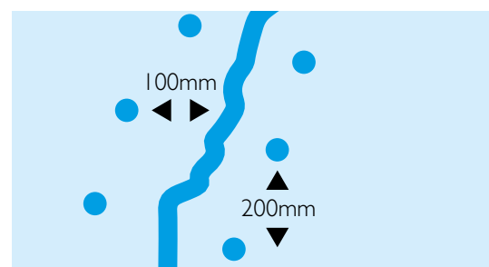
Figure 2B: Vertical view of a crack showing the ideal positioning of the drilled holes when preparing for the injection of crack filling
