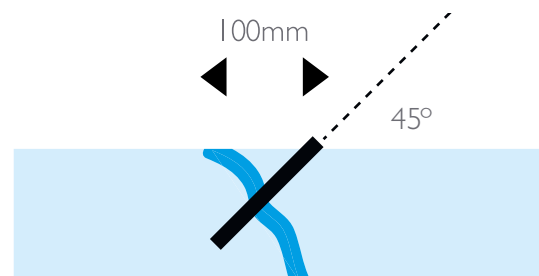
Figure 2A: Cross-section view showing the correct drilling of holes when preparing for crack injection
