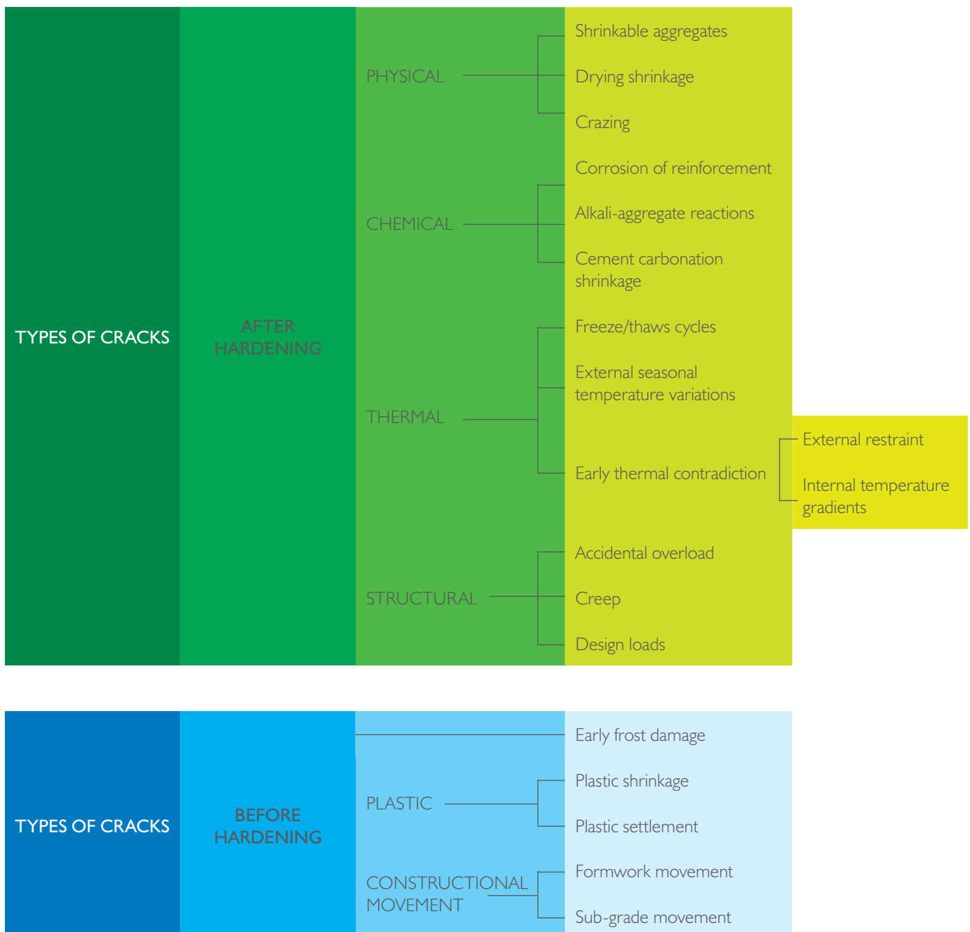
Figure 1: Types of cracks and their causes
